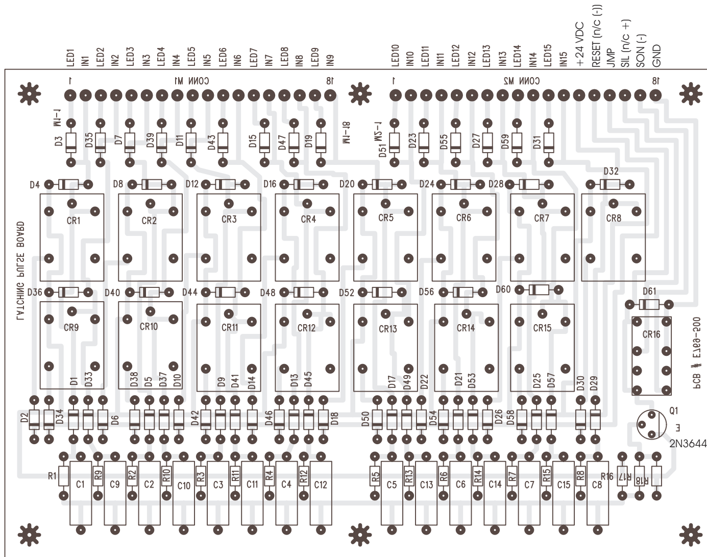
NEGATIVE-INPUT PULSE/LATCH BOARD PCB # E769-500 see schematic # E769-50N
