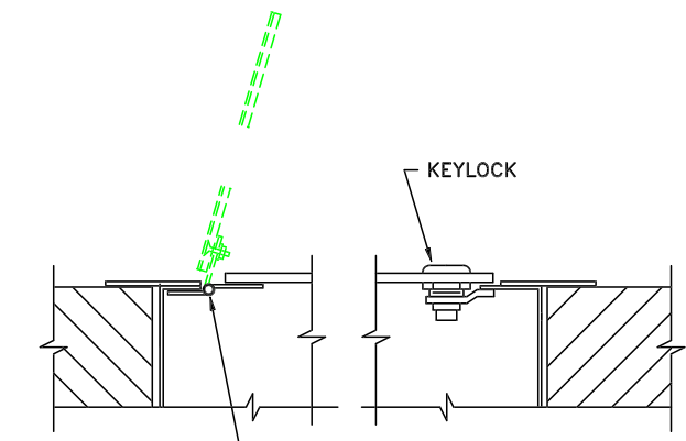
CROSS SECTION (ASSEMBLED VIEW)
