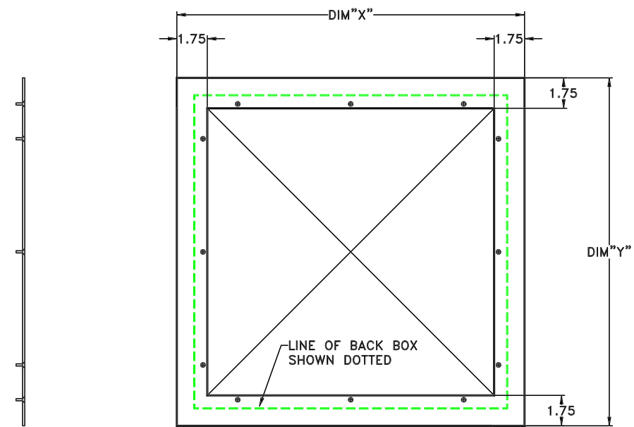
TRIM RING 14 GA. CRS
