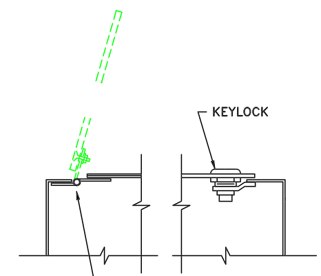
CROSS SECTION (ASSEMBLED VIEW)
