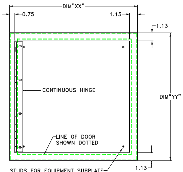
BACK BOX FRONT VIEW 16 GA. CRS
