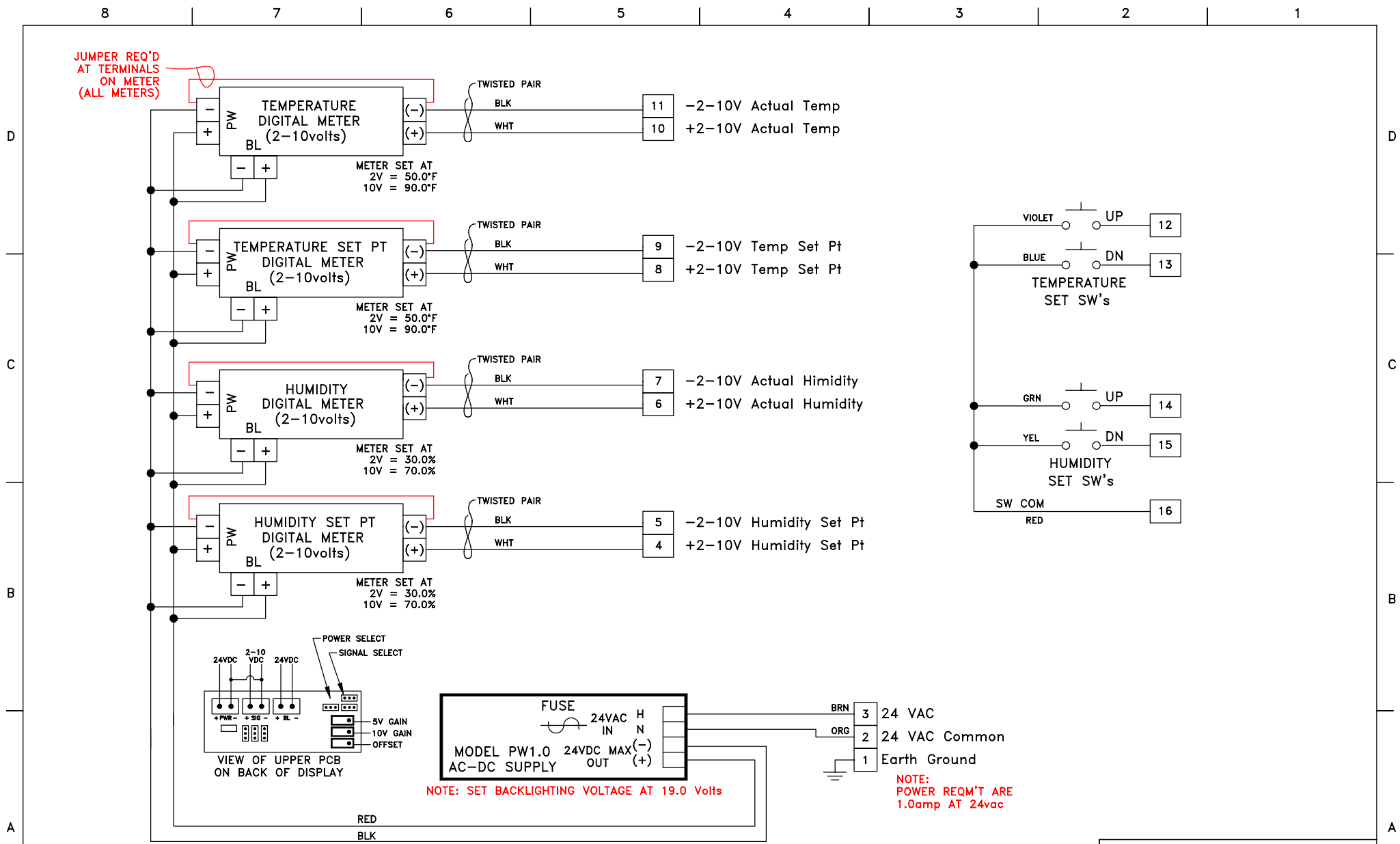
WIRING DETAILS FOR COMPONENTS WIRED TO TERMINALS
